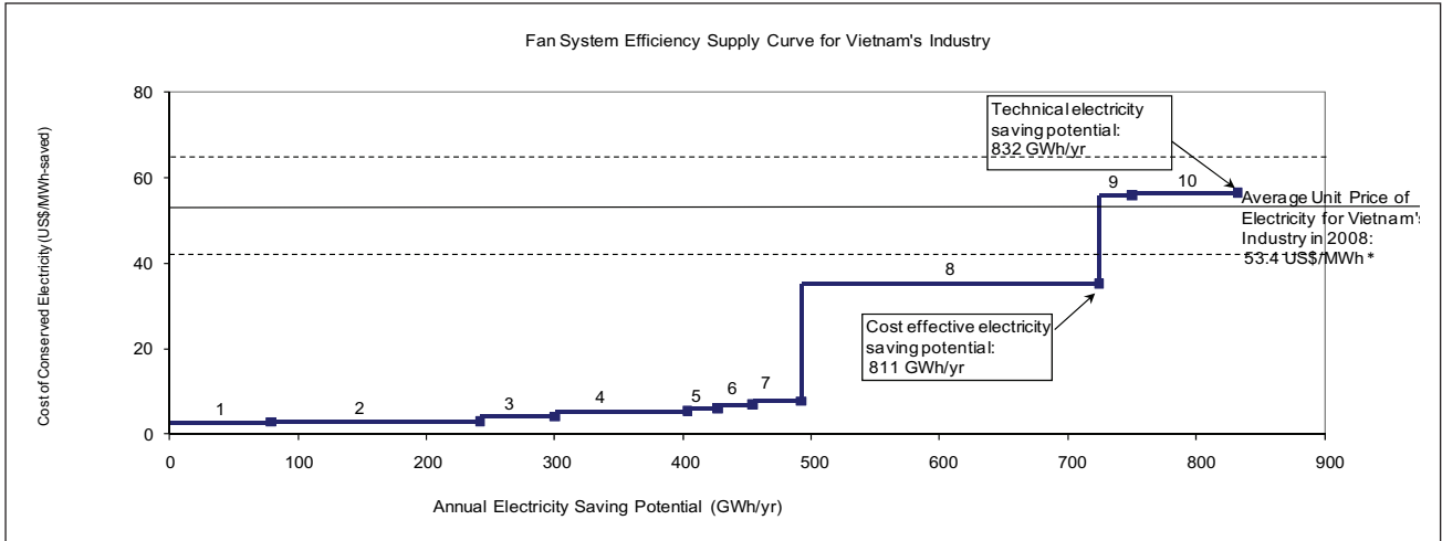
Figure 20: Vietnam's Fan System Efficiency Supply Curve
