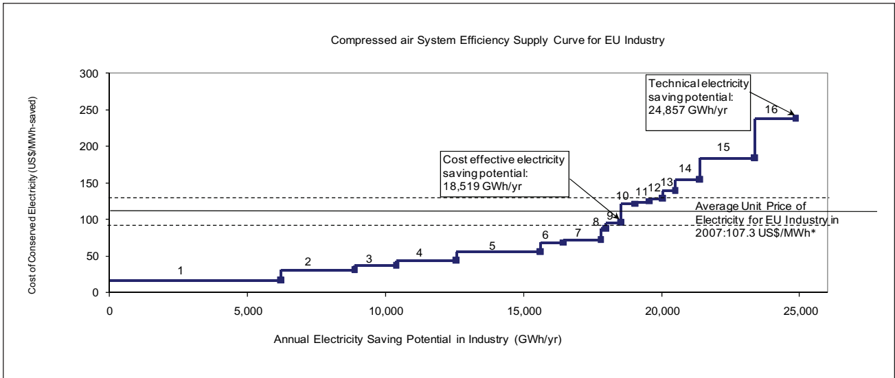
Figure 12: EU's Compressed Air System Efficiency Supply Curve
