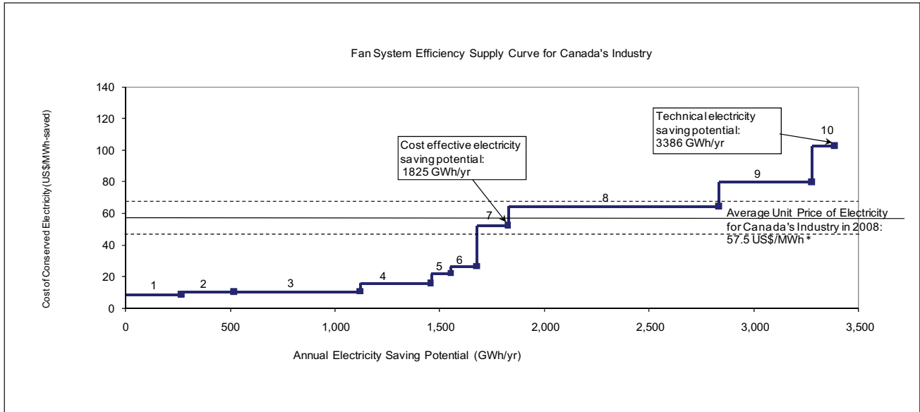
Figure 17: Canada's Fan System Efficiency Supply Curve
