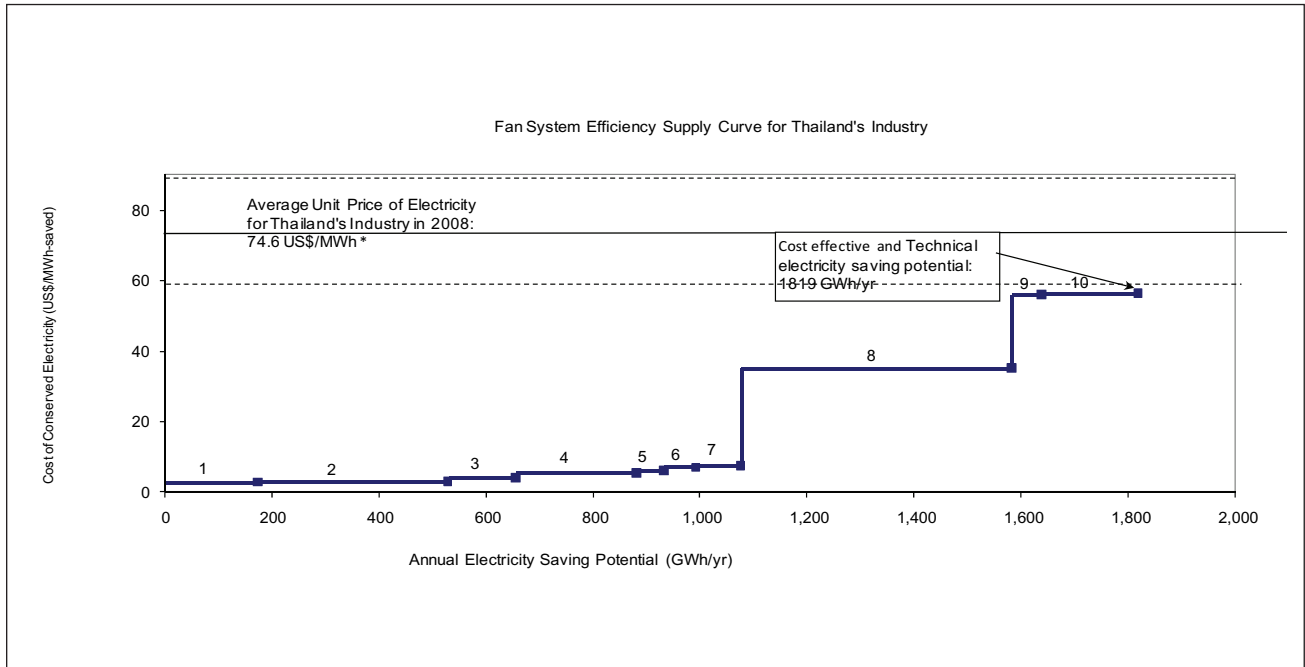
Figure 19: Thailand's Fan System Efficiency Supply Curve
