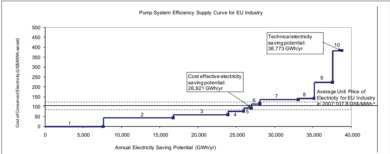
Figure 6: EU's Pumping System Efficiency Supply Curve
