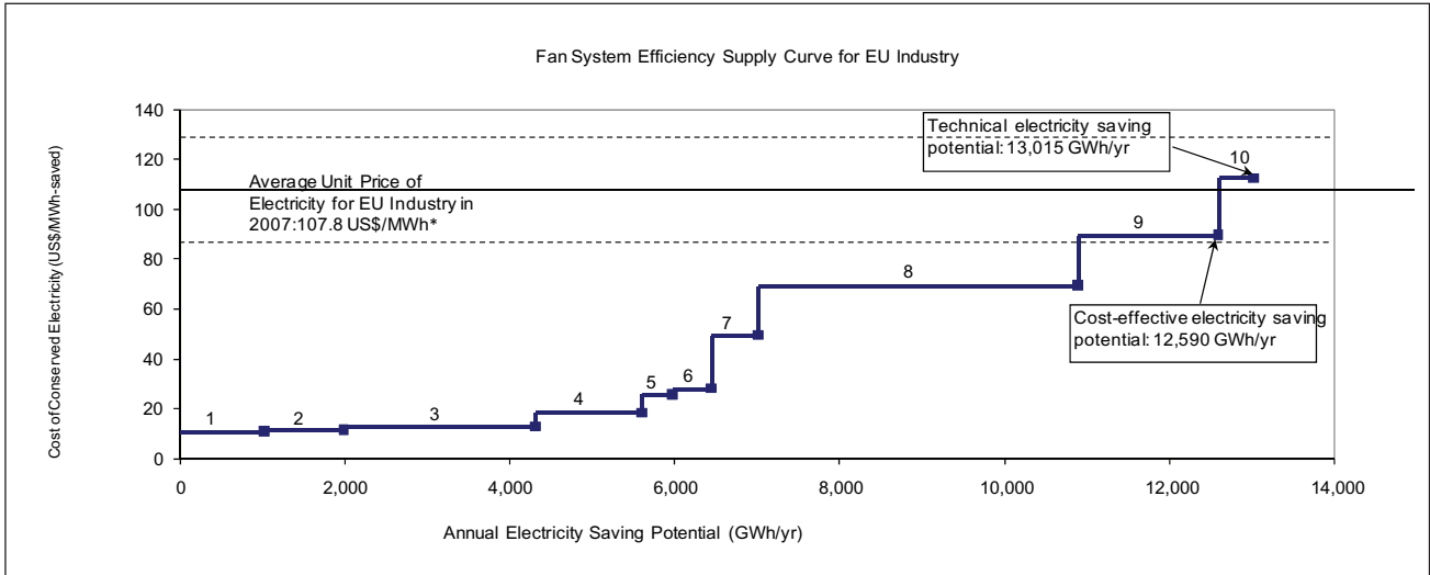
Figure 18: EU's Fan System Efficiency Supply Curve
