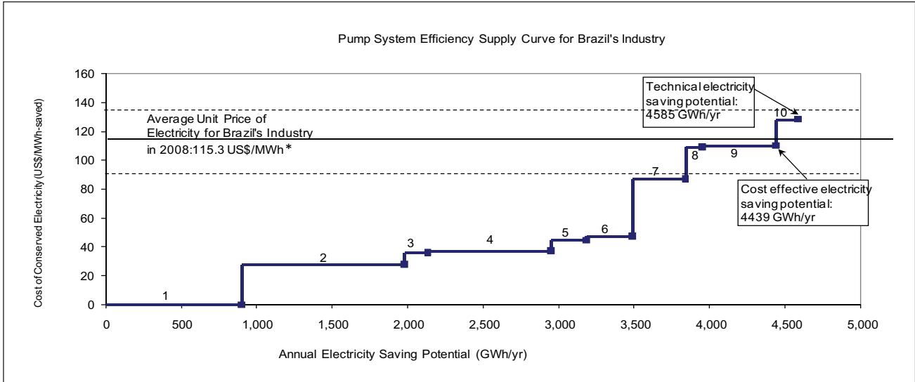
Figure 9: Brazil's Pumping System Efficiency Supply Curve
