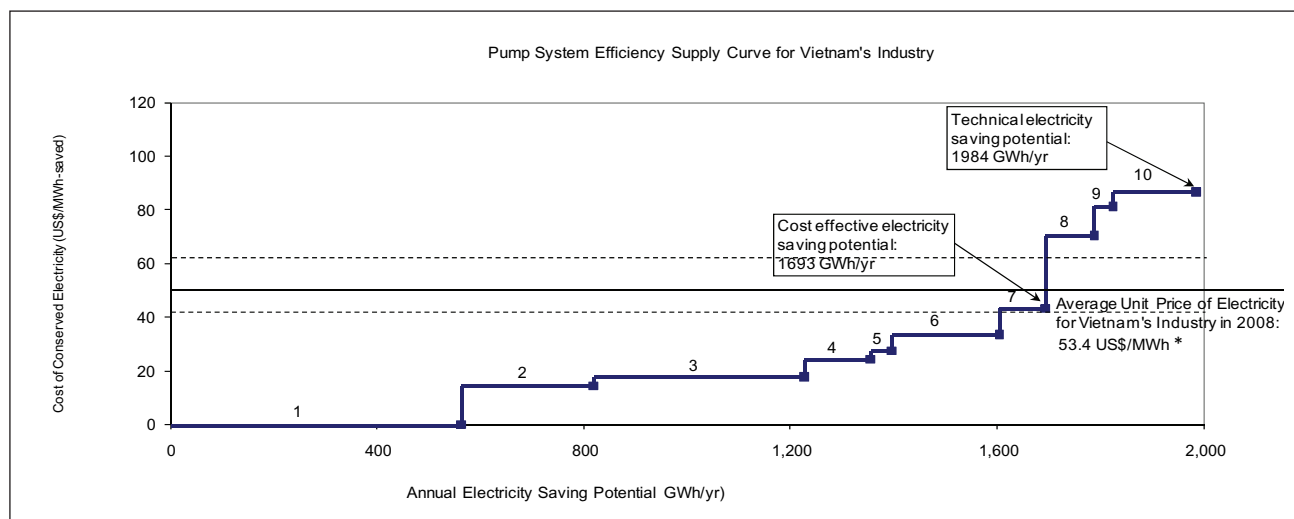
Figure 8: Vietnam's Pumping System Efficiency Supply Curve
