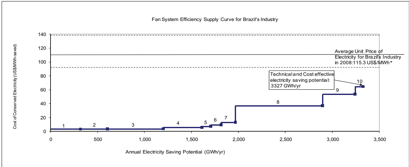
Figure 21: Brazil's Fan System Efficiency Supply Curve
