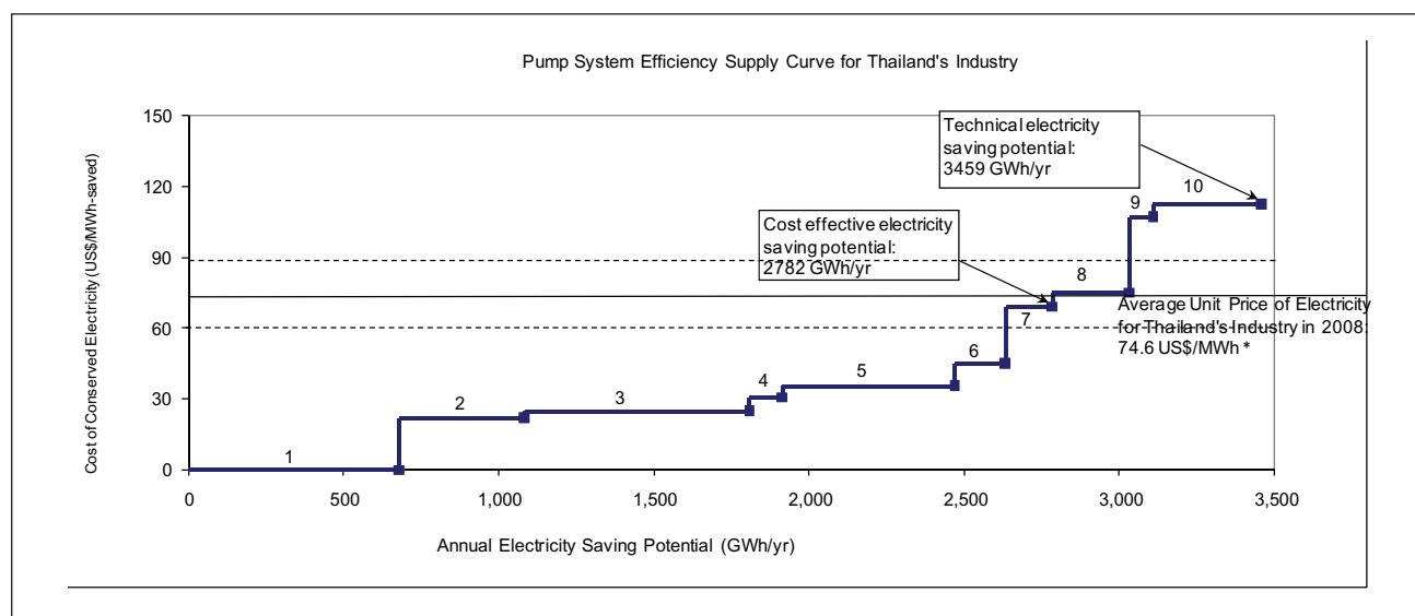
Figure 7: Thailand's Pumping System Efficiency Supply Curve
