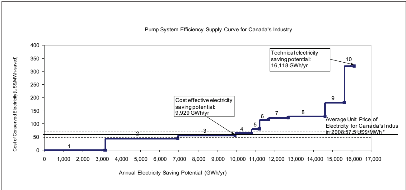
Figure 5: Canada's Pumping System Efficiency Supply Curve
