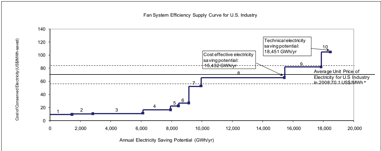
Figure 16: US Fan System Efficiency Supply Curve
