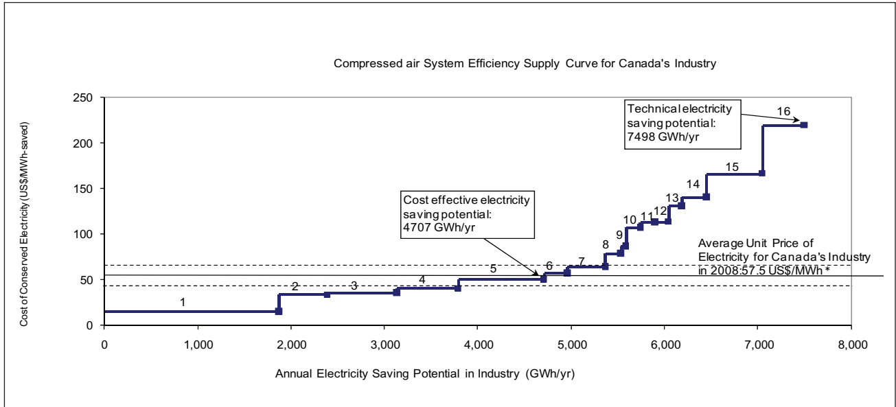
Figure 11. Canada's Compressed Air System Efficiency Supply Curve
