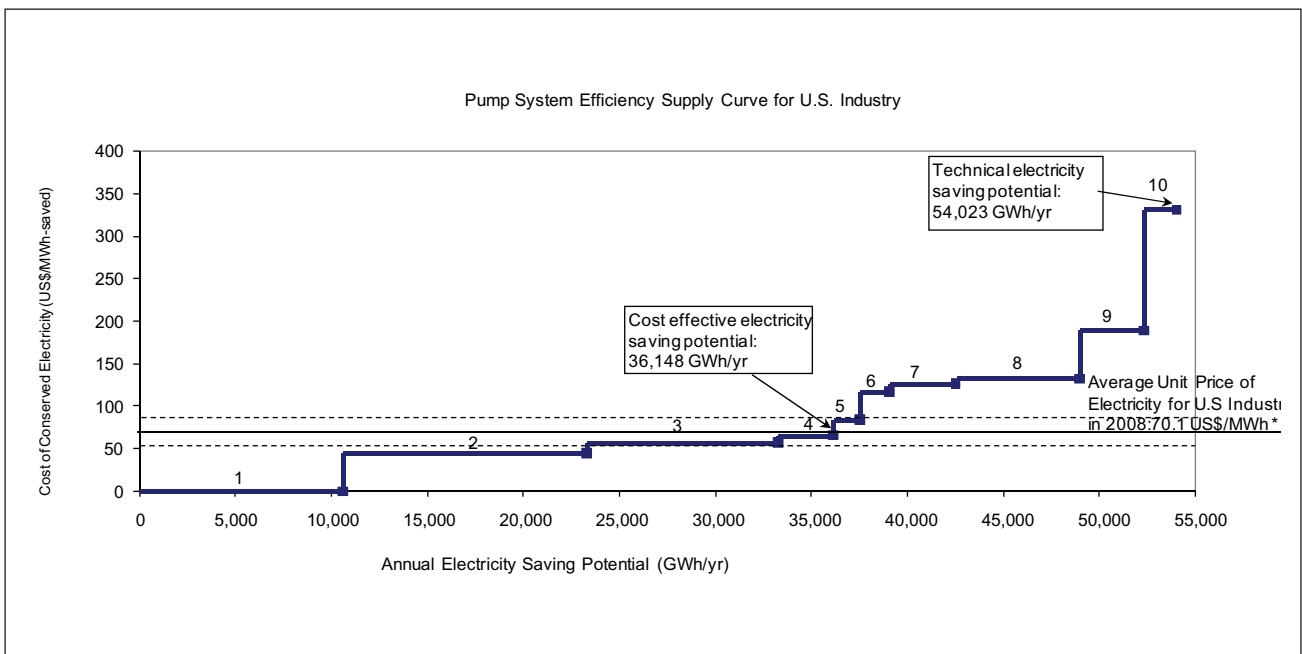
Figure 4: US Pumping System Efficiency Supply Curve
