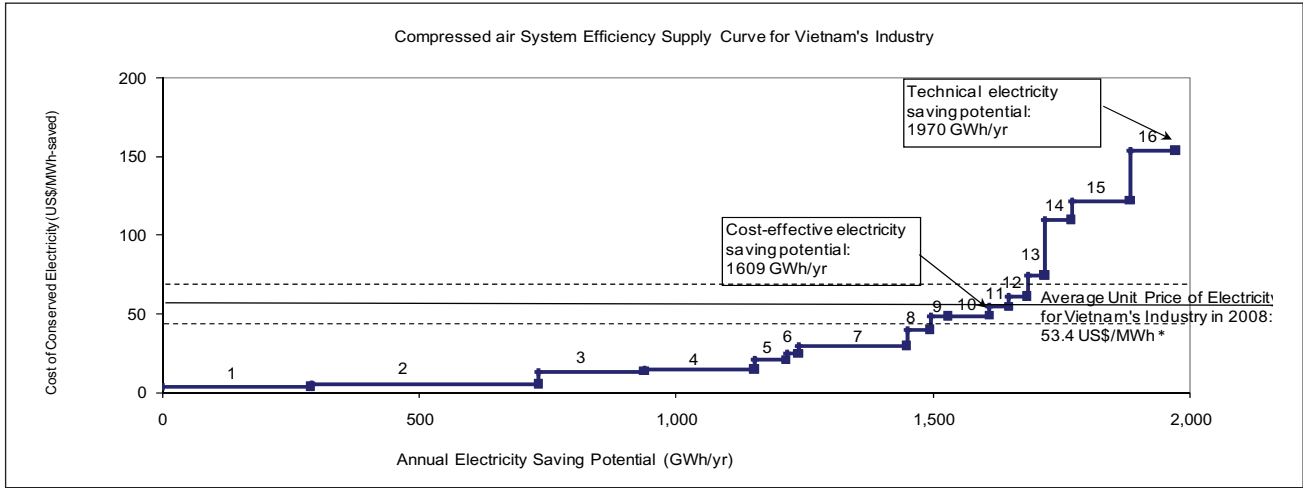
Figure 14: Vietnam's Compressed Air System Efficiency Supply Curve
