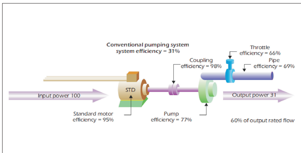
Figure 1: Conventional Pumping System Schematic (Almeida, et al., 2005.)
