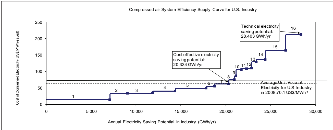
Figure 10: US Compressed Air System Efficiency Supply Curve
