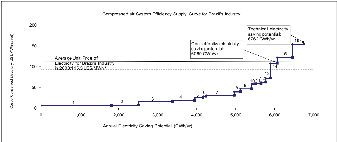
Figure 15: Brazil's Compressed Air System Efficiency Supply Curve
