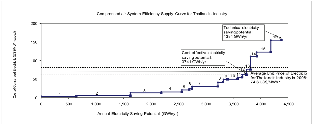
Figure 13. Thailand's Compressed Air System Efficiency Supply Curve
